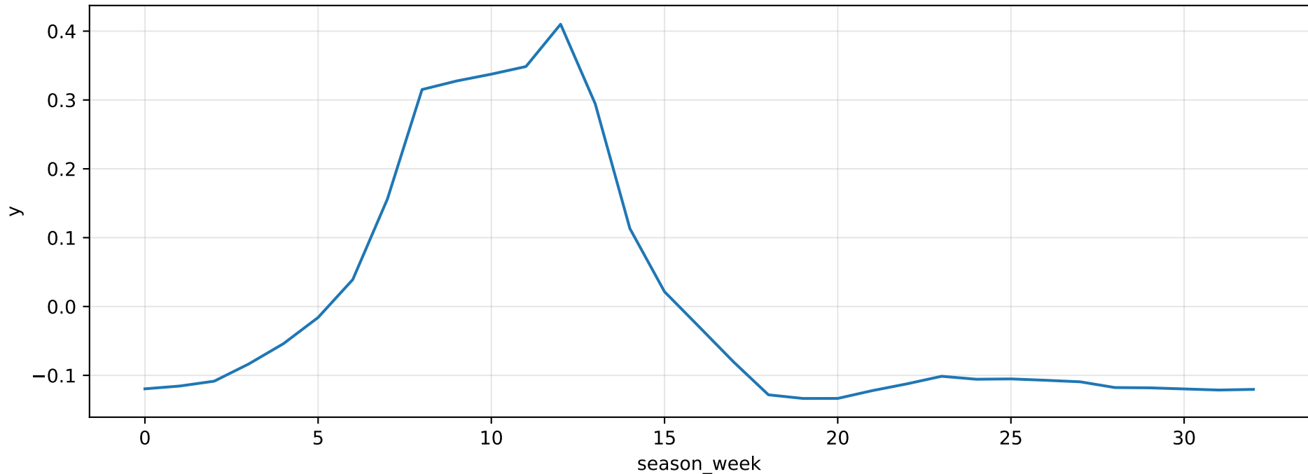
Z-score normalized PCA: U2
