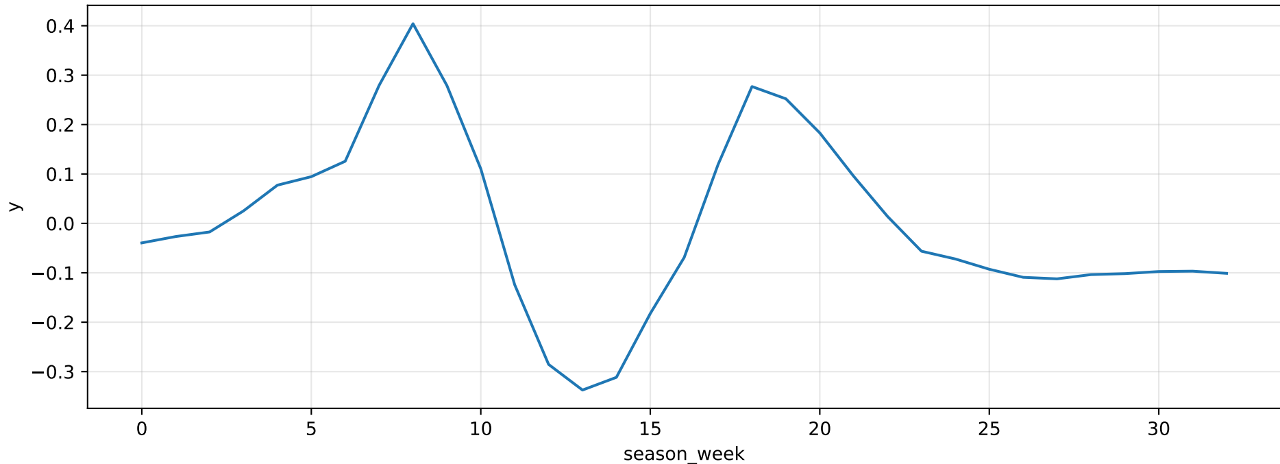
Z-score normalized PCA: U3
