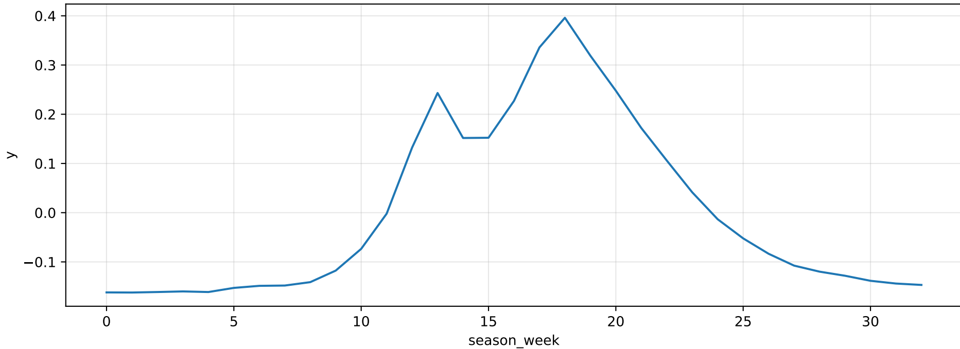
Z-score normalized PCA: U1
