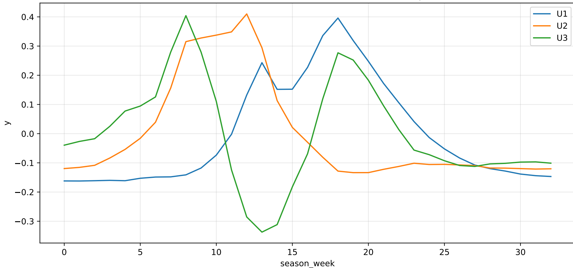
Z-score normalized PCA: First U vectors (overlay)
