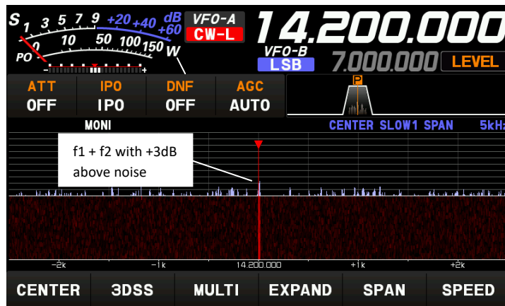
Figure 12: DR2 interference signal at P_i = -22\text{dBm} , IPO
