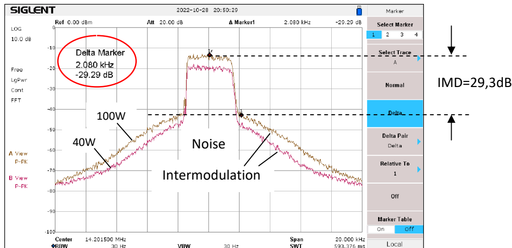
Figure 21: Transmitter noise signal at 100 watts (yellow) and 40 watts (purple), 14.2MHz (SSB)
