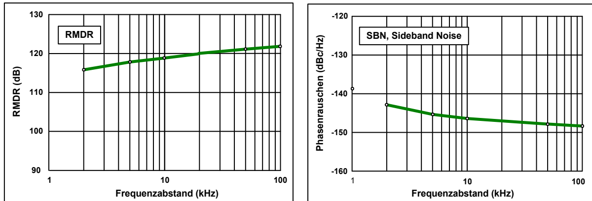
Figure 6: RMDR (left) and phase noise (right) at a distance of 2kHz to 100kHz from the carrier
