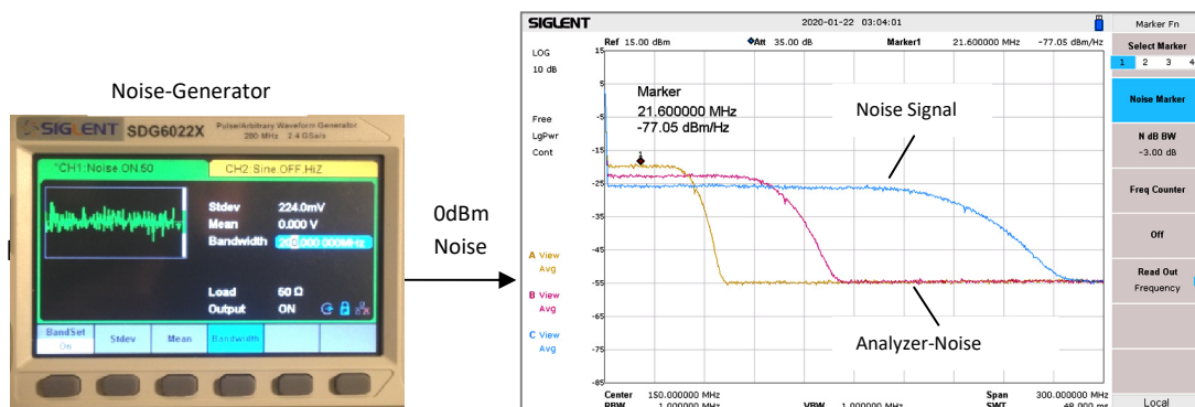
Figure 15: Noise signal with 0dBm power at 50MHz, 100MHz and 200MHz noise bandwidth
