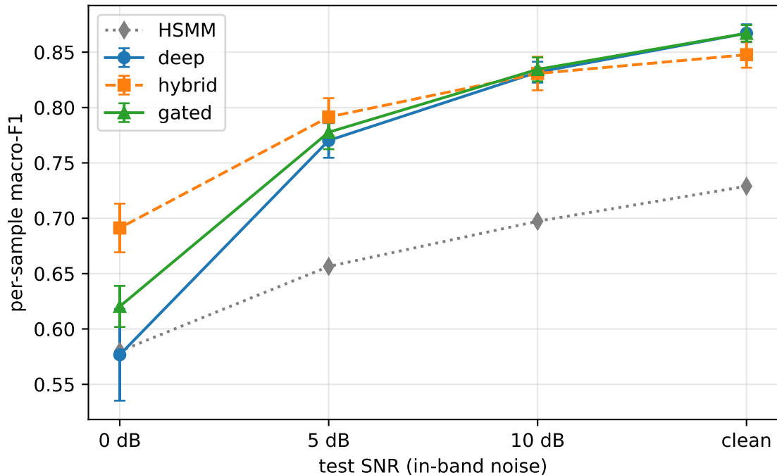
Noise robustness: deep vs hybrid vs gated
