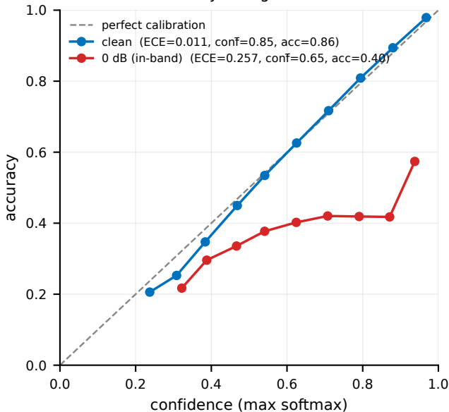
Deep is well-calibrated when clean, confidently wrong under noise
