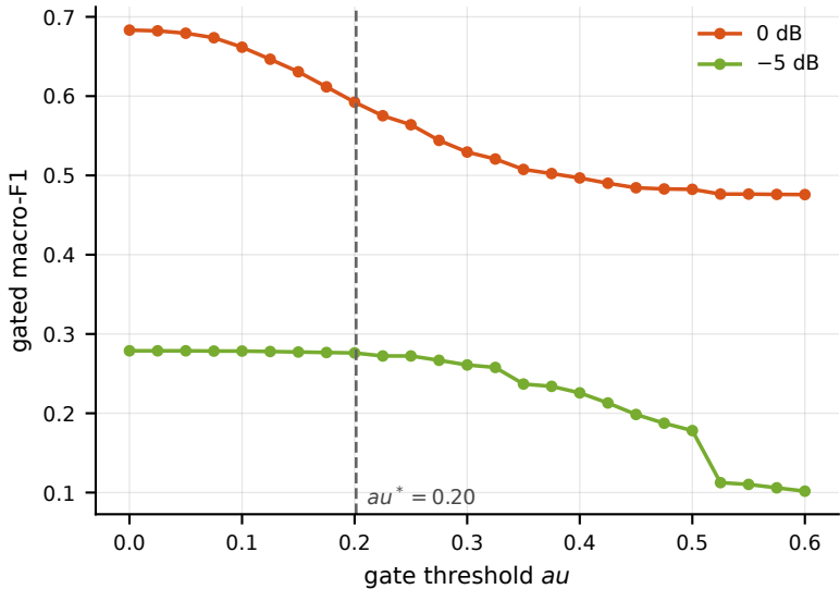
Gate-threshold sensitivity (5 seeds)
