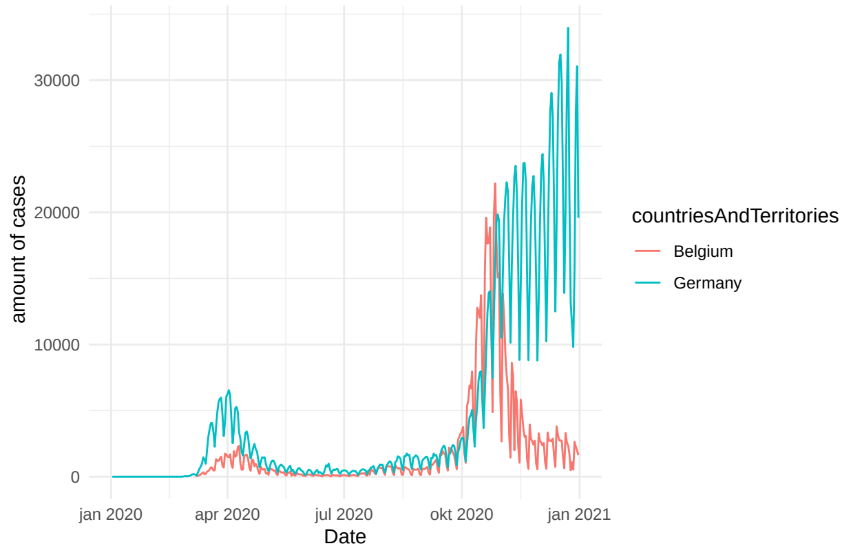
COVID-19 cases in selected countries in time 2020
