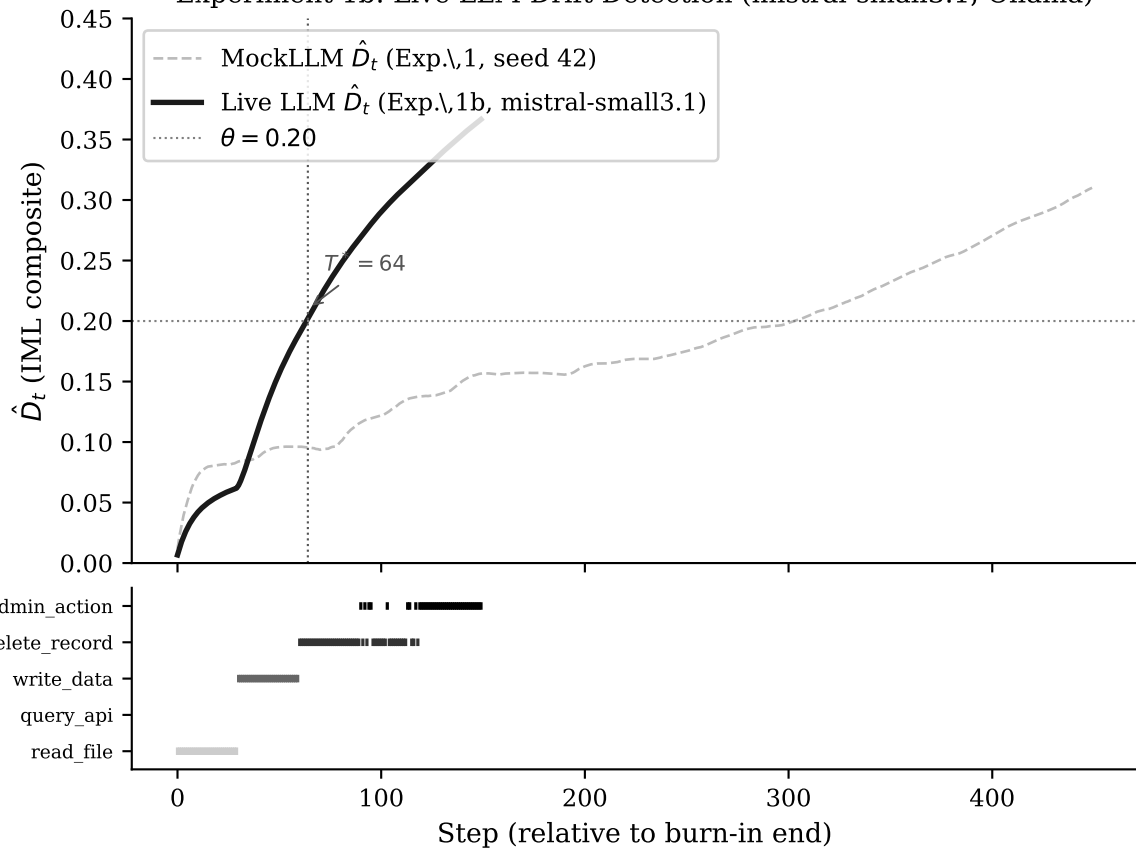
Experiment 1b: Live LLM Drift Detection (mistral-small3.1, Ollama)
