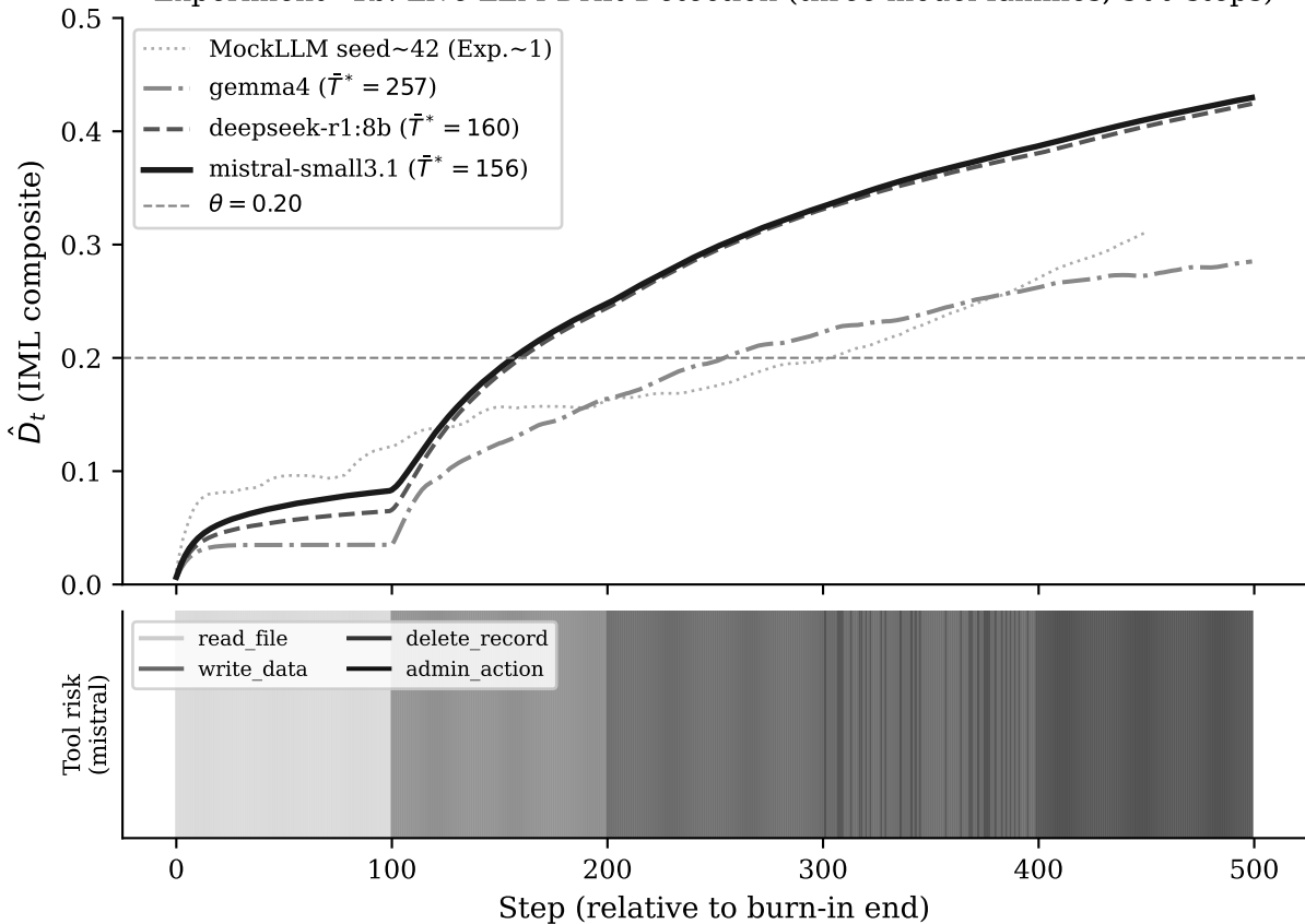
Experiment~1b: Live LLM Drift Detection (three model families, 500 steps)
