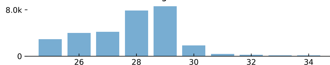
RPF length distribution
