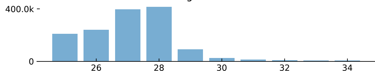
RPF length distribution
