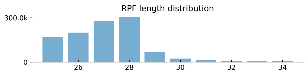
5' end match RPFs
