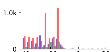
RPF near stop codon
