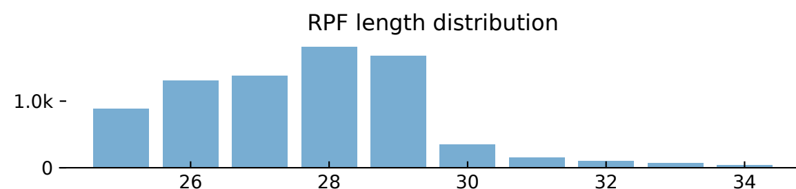
5' end mismatch RPFs
