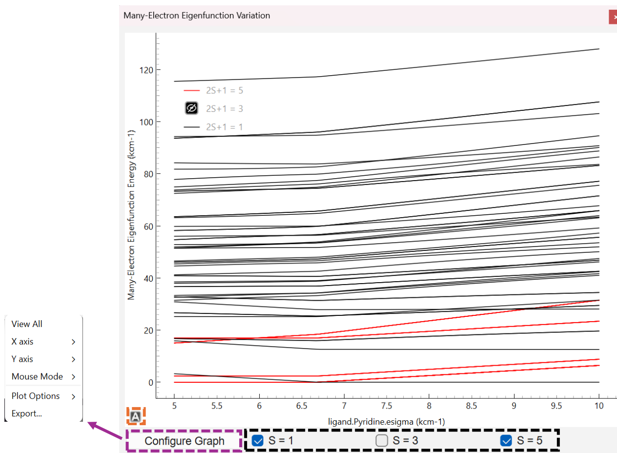
Figure 4: Variation plot of many-electron eigenfunctions for a d^6 \text{Fe}^{2+} complex 2 showing the energies of singlet and quintet states, with the triplet states hidden. Note that spin-crossover from the low-spin ( 2S+1=1 ) to high-spin ( 2S+1=5 ) states can be seen at around 6500 \text{ cm}^{-1} .
