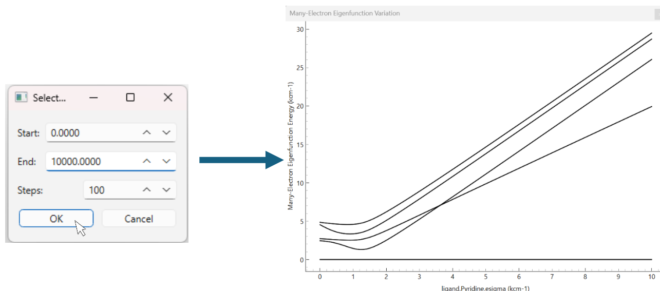
Figure 3: Variation plot of many-electron eigenfunctions for [\text{Cu}(\text{py})_4]^{2+} . 5 states in total are observed as expected for a d^9 system, with their energies tending to increase in energy as the strength of pyridine \sigma donation increases.
