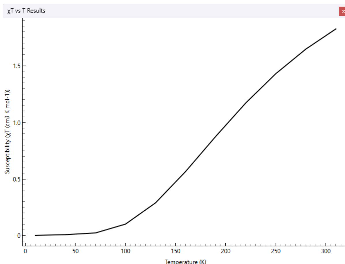
Figure 15: Paramagnetic susceptibility curve plotted from the data in figure 14.
