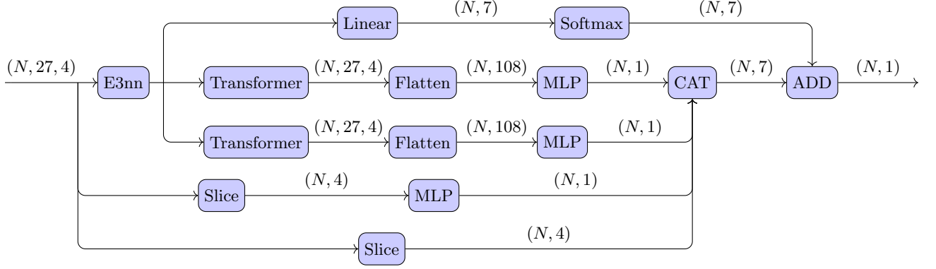
FIG. 1: The architecture of the neural network. We use the E3nn block [?] to extract the invariant features from the input, and the Slice block is used to extract the energy density at the center ( e(\mathbf{r}_i) ), which is already the invariant feature, from the input. The transformer we use here is only composed of multilayer of the scaled dot-product attention part of the original transformer [1]. Other information about the architecture of the neural network is described in the appendix.
