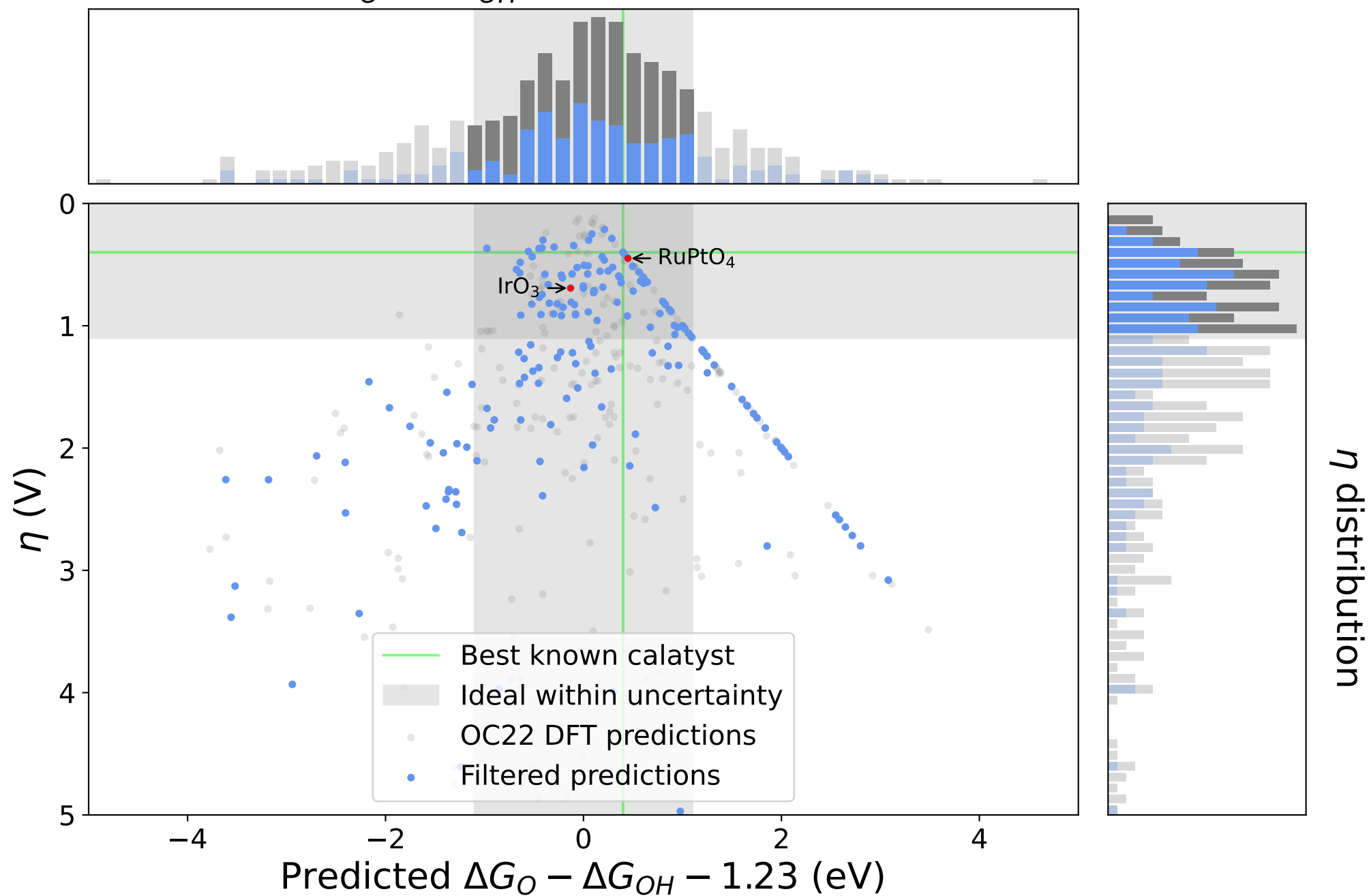
\Delta G_O - \Delta G_{OH} - 1.23 distribution
