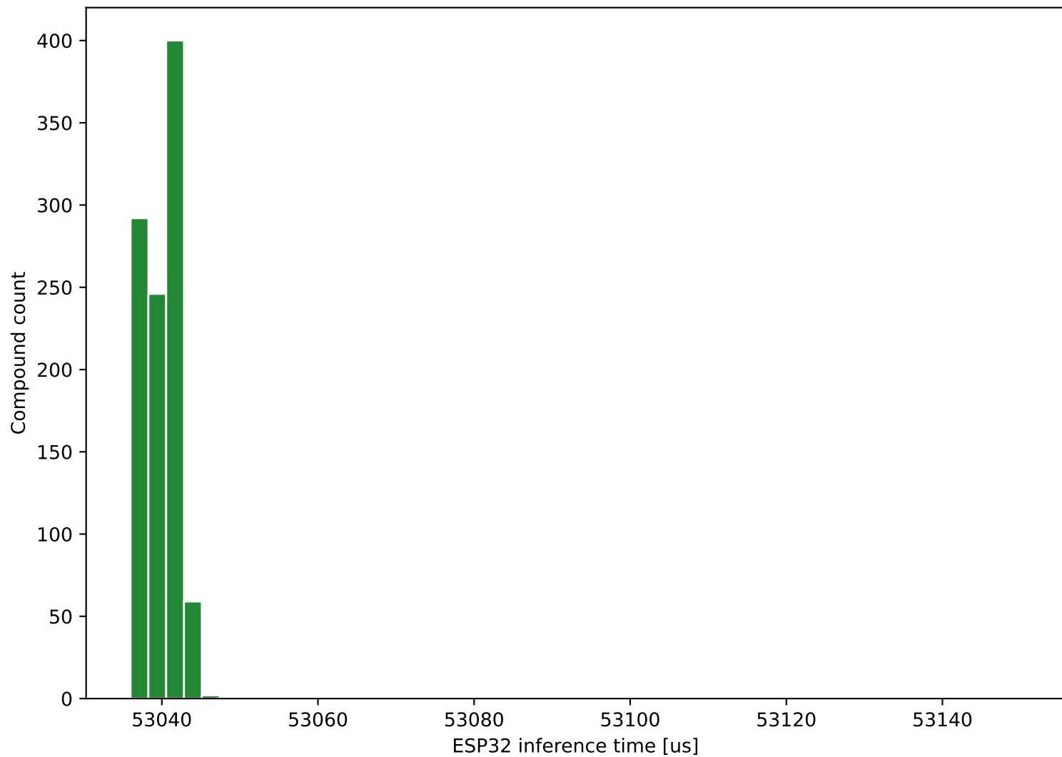
On-device inference time distribution
