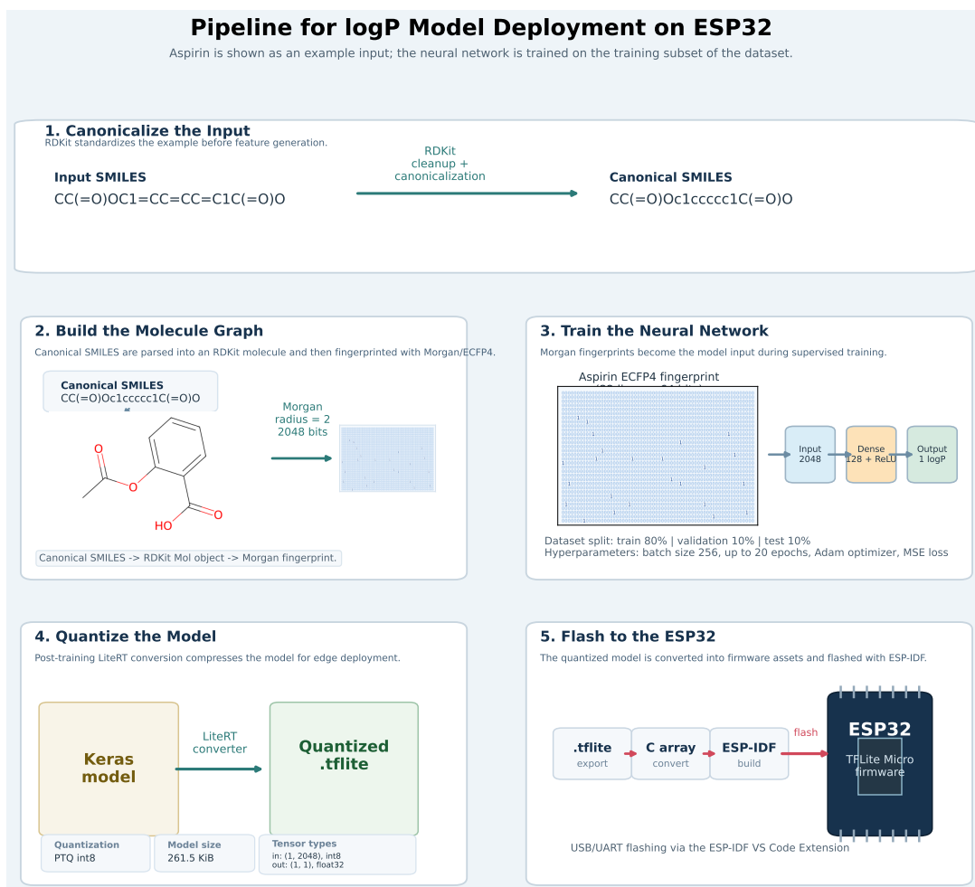
Figure 2.2: Workflow diagram showing the stages of canonicalization, fingerprint generation, neural network training, quantization, and ESP32 deployment.
