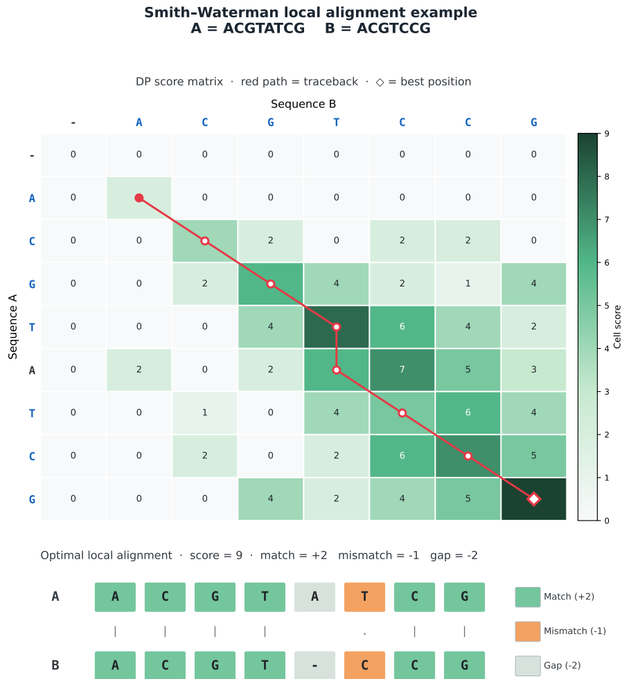
Figure 2: Example of a local alignment between two DNA sequences, as produced by the Smith-Waterman algorithm.
