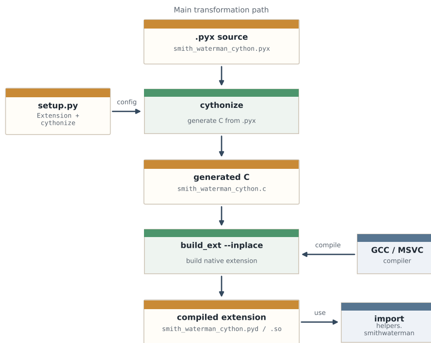
Figure 1: The Cython build pipeline, from a .pyx file to a compiled extension module.
