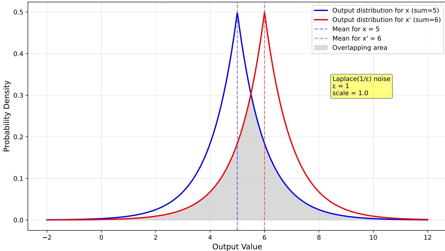
Differential Privacy: Output Distributions with Laplace Noise ( \epsilon = 1 )
