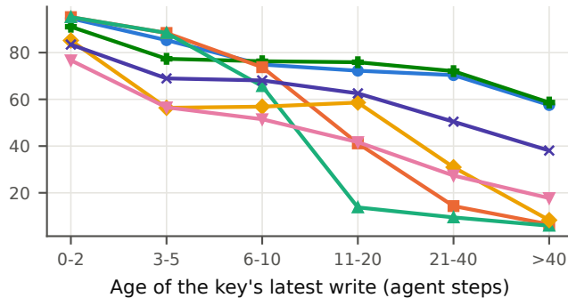
State probes at 8k: correct (%)
