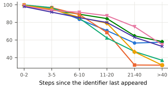
Use probes at 8k: available (%)
