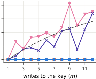
budget 8k (random keeps \rho=0.08 )
