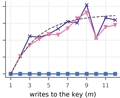
budget 32k (random keeps \rho=0.29 )
