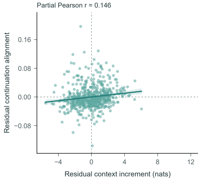
b Adjusted for word-only preference
