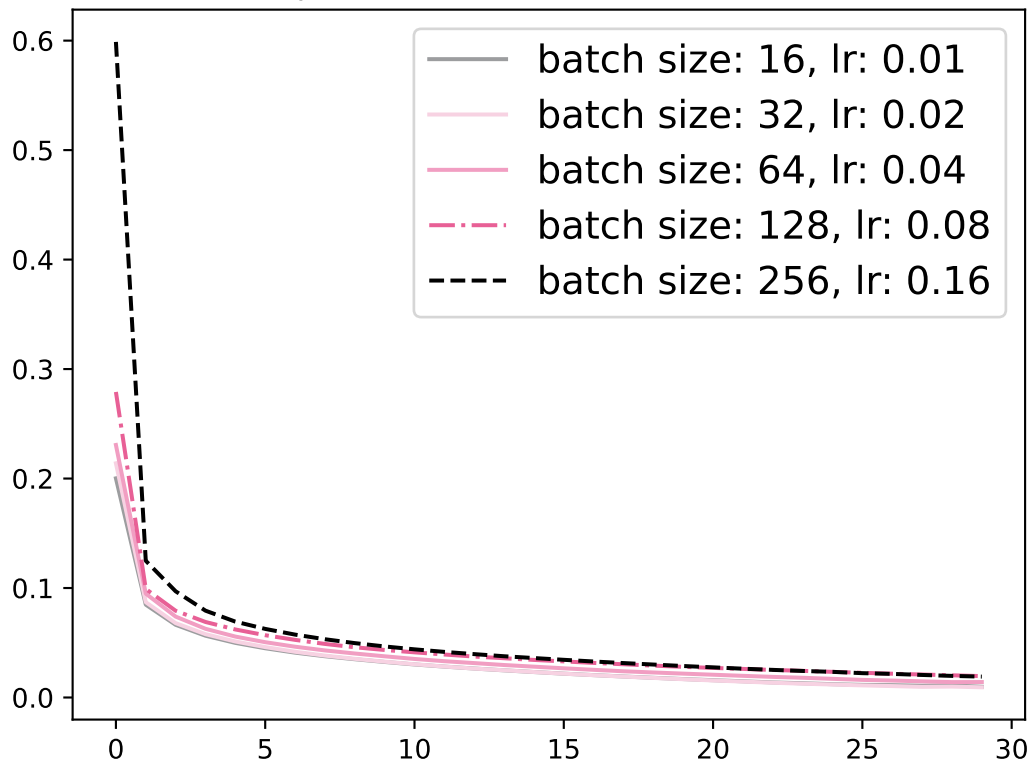
epoch loss with different bs and lr
