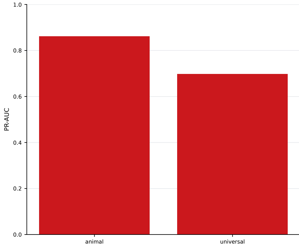
Pair ranker
