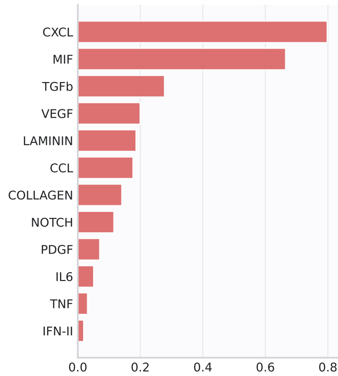
Differential pathway rank
