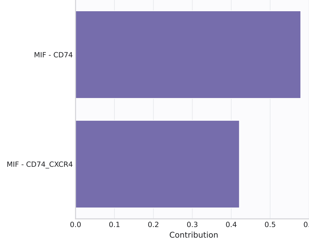
MIF LR contribution
