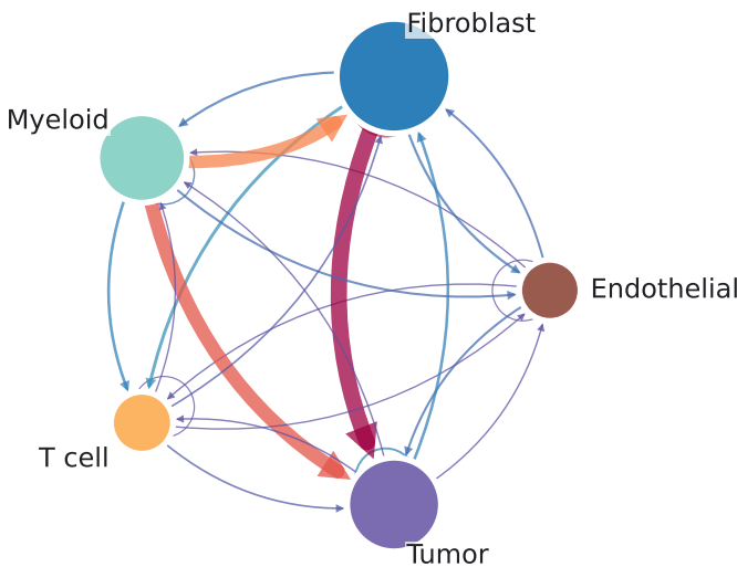
Individual LR circle
