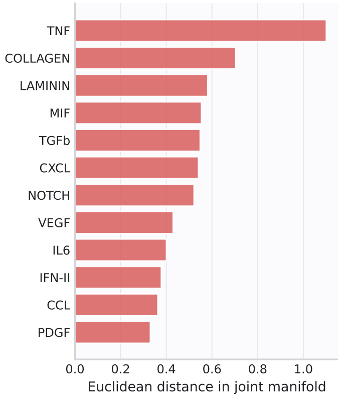
Pathway distance rank
