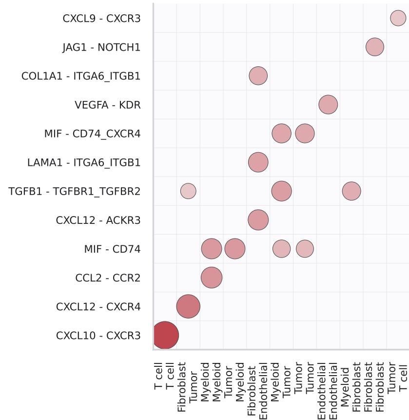
Pathway distance rank
