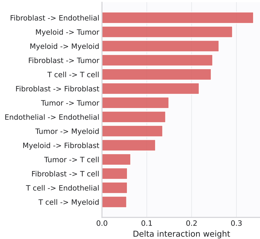
Differential source-target rank
