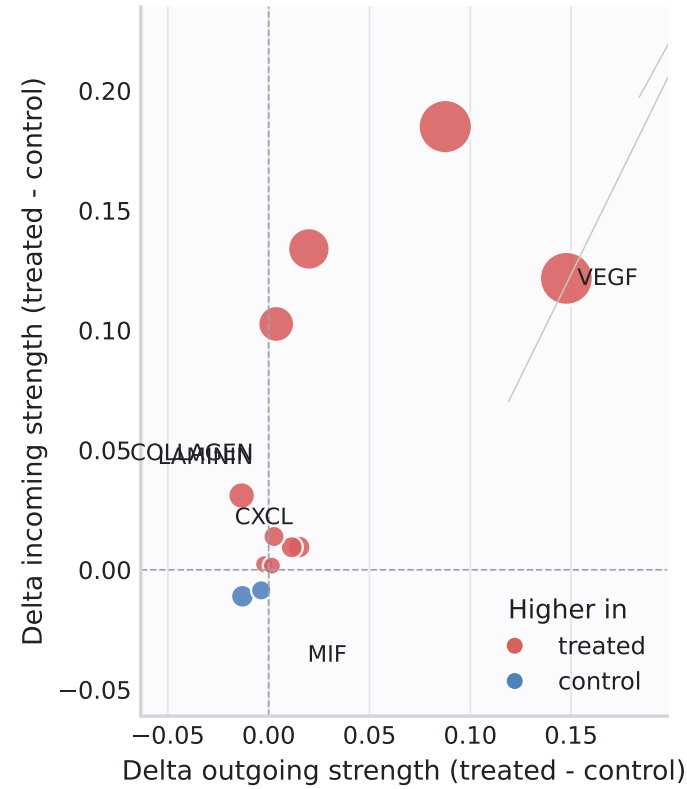
Signaling changes: Endothelial
