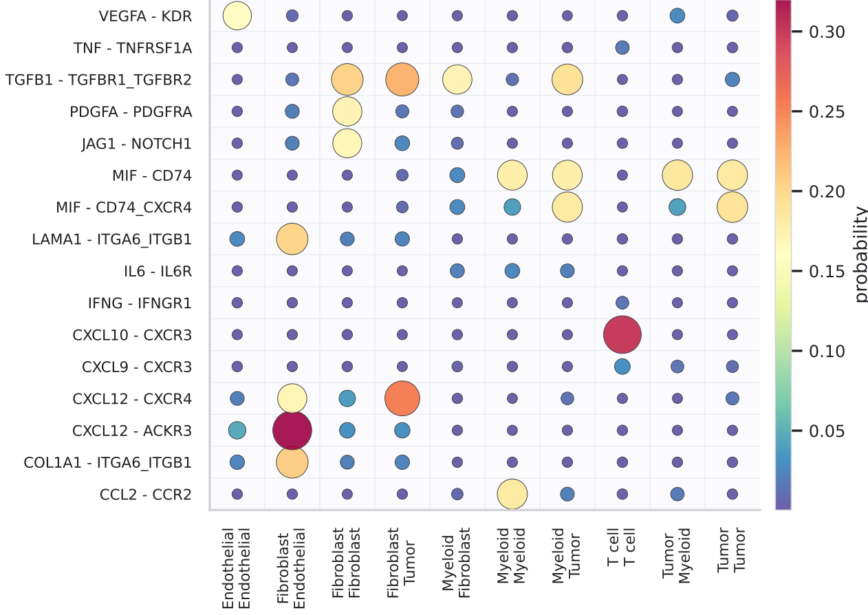
Top LR programs
