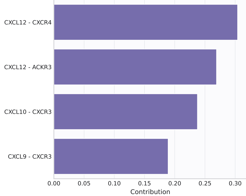
CXCL LR contribution
