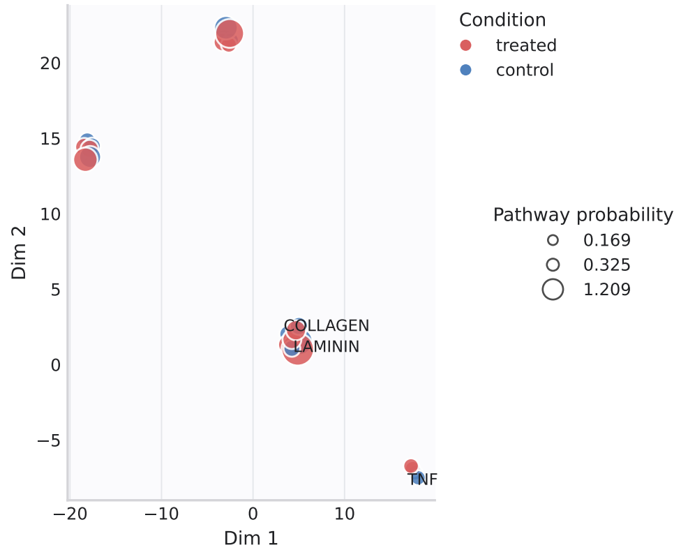
Pairwise pathway embedding
