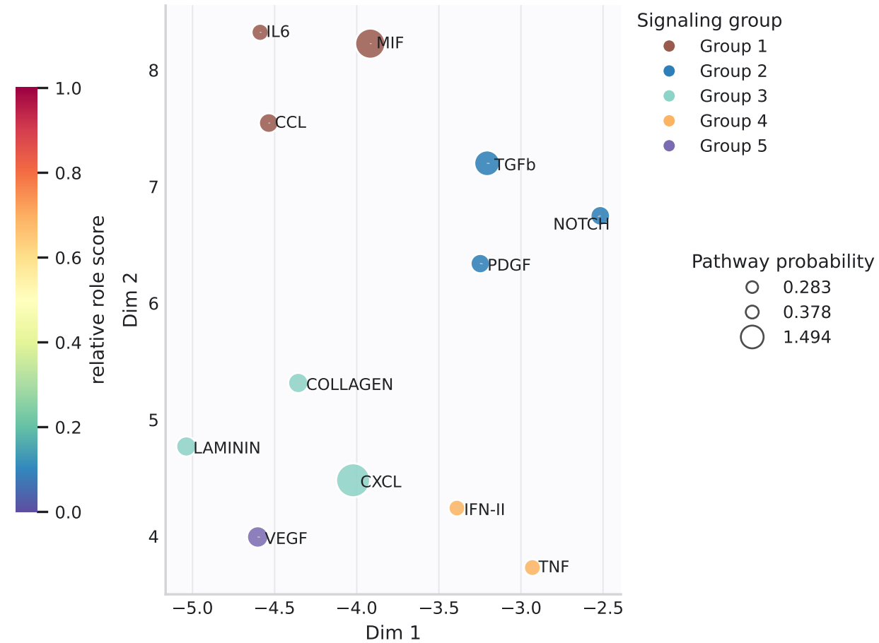
Pathway embedding groups
