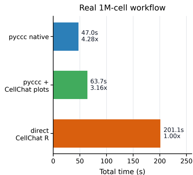
Figure 1. pyccc keeps CellChat-like CCC in an AnnData-native sparse workflow, matches CellChat R numerics on the official tutorial benchmark, accelerates the real 1M-cell workflow by avoiding CellChat's dense cell-level path, and exposes outlier-robust summary options with explicit similarity tradeoffs.
