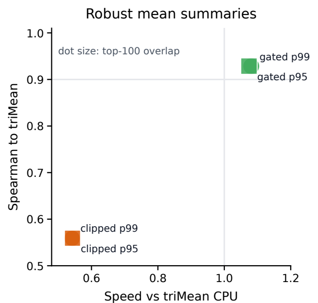
Figure 1. pyccc keeps CellChat-like CCC in an AnnData-native sparse workflow, matches CellChat R numerics on the official tutorial benchmark, accelerates the real 1M-cell workflow by avoiding CellChat's dense cell-level path, and exposes outlier-robust summary options with explicit similarity tradeoffs.
