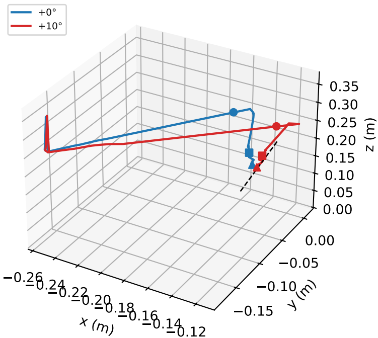
Figure 1 — actual peg-tip trajectories (block 0): 0^\circ vs +10^\circ pitch
