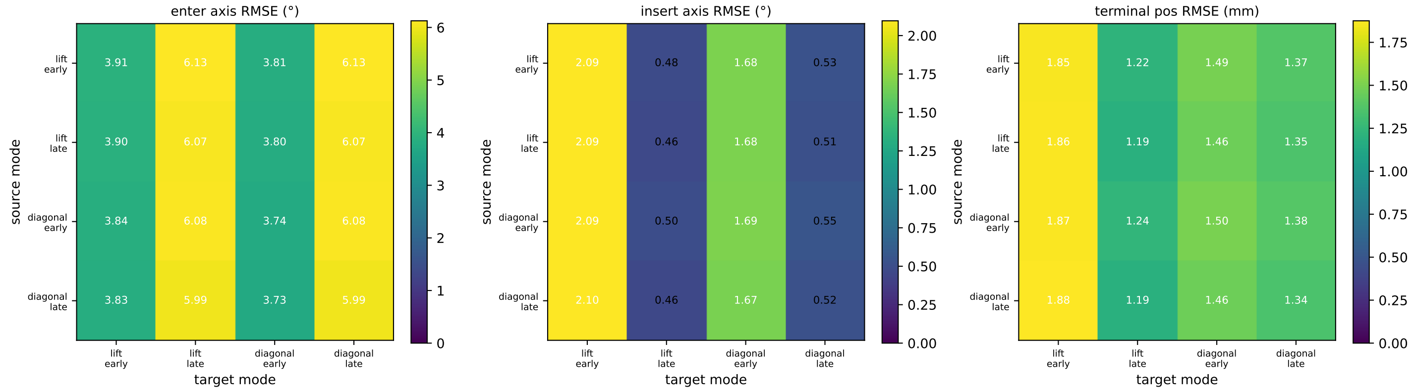
Figure 3 — 4×4 source→target held-out error (method = frozen source law)
