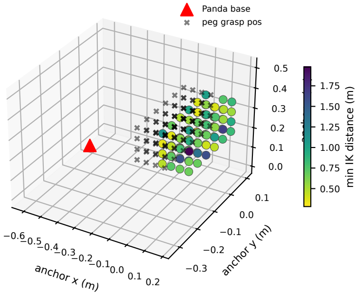
Q2_Ry90: 3D feasibility (color = IK dist)
