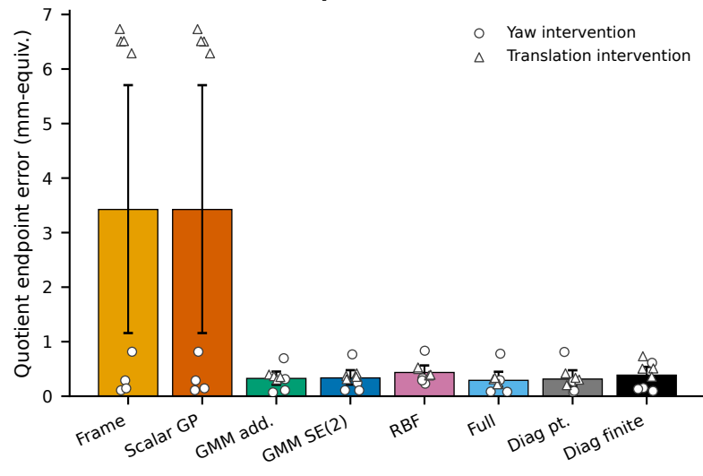
D Held-out task-endpoint error
