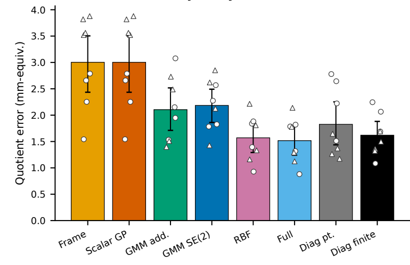
C Held-out task-trajectory error
