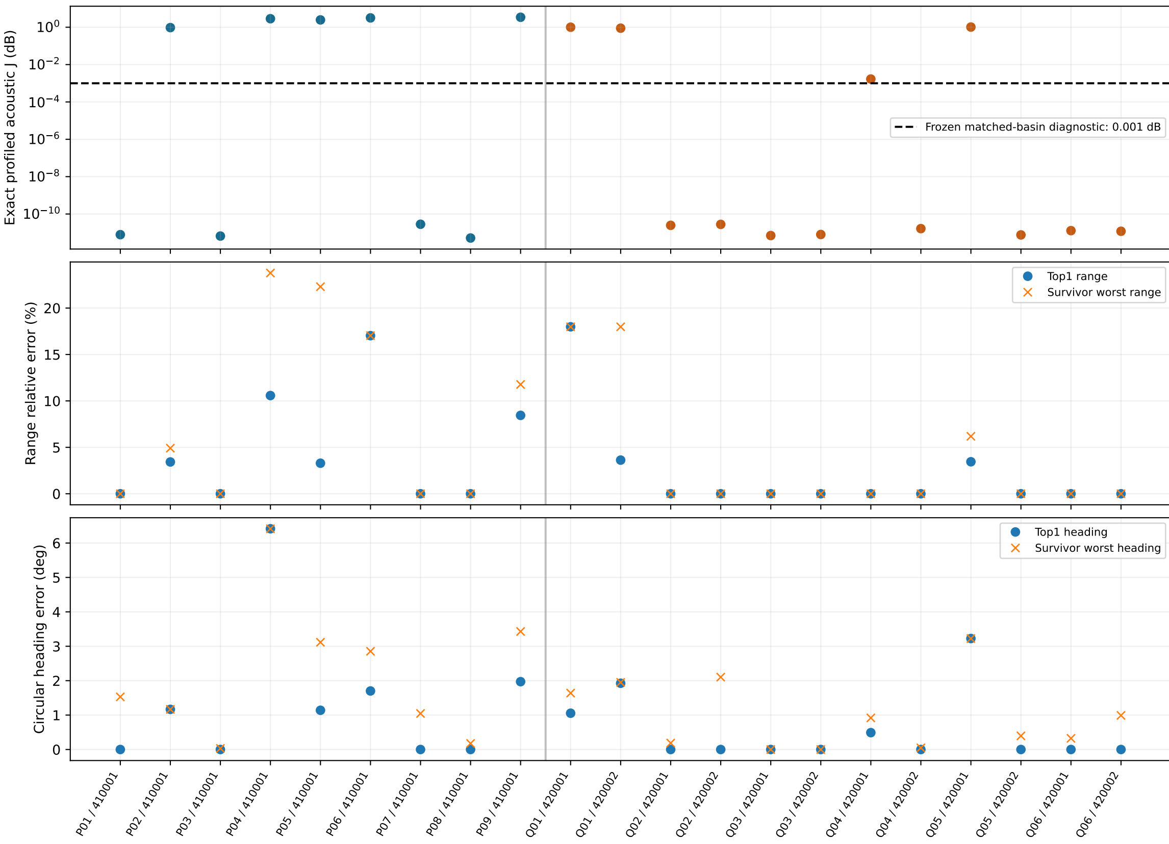
R4-A1-FIX V2: fixed-budget continuous search at nominal 0.1 deg 9 regression cases (blue) + 12 preregistered holdout cases (orange); no sensor-tolerance claim
