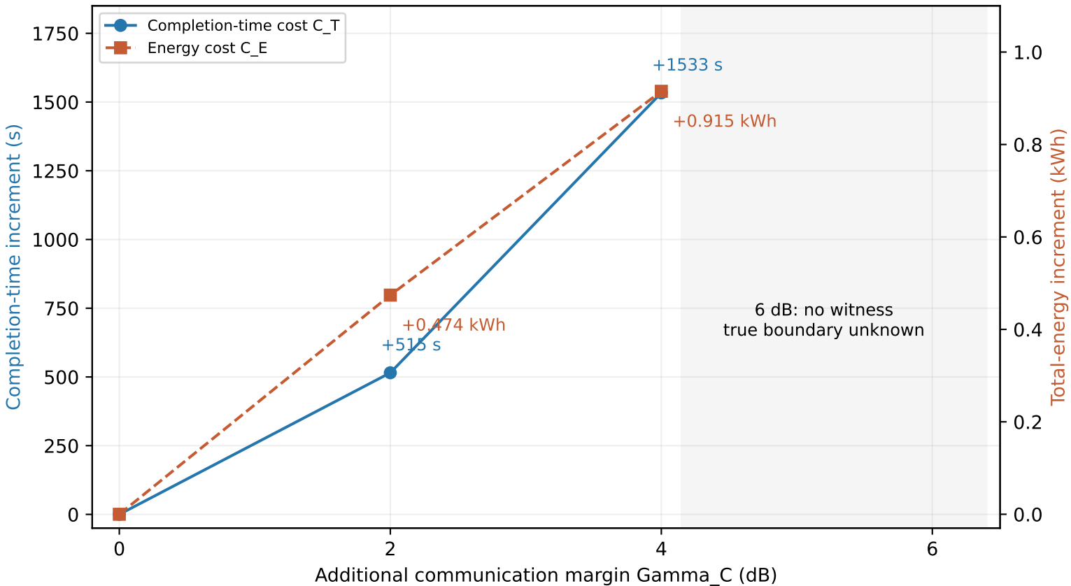
Achievable robustness costs at a common lateness budget of 1,000,000
