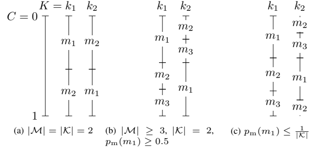
Figure 8: p_k -agnostic scheme for any key distribution p_k
