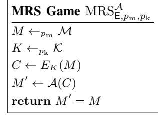
Figure 5: Game for message recovery security (MRS)
