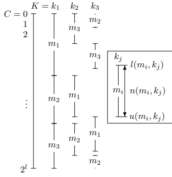
Figure 6: Ciphertext intervals in OE
