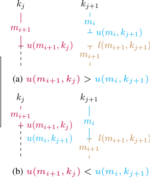
Figure 6: Ciphertext intervals in OE
