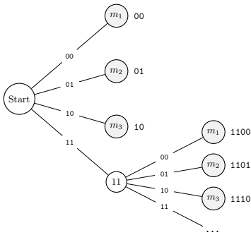
Figure 9: The infinite prefix tree illustrating how a variable-length homophonic encoder maps codewords to messages m_1, m_2, m_3 under a uniform distribution (\frac{1}{3}, \frac{1}{3}, \frac{1}{3}) . The tree continues to expand infinitely along the 11 branches.
