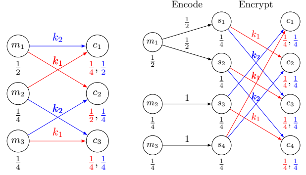
(a) Deterministic cipher (b) Homophonic cipher (HC) / honey encryption (HE) with n(m, k) \propto p_m(m) .
