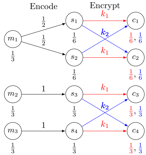
Figure S.3: Counterexample to the converse of Theorem 3: p_{\mathbf{m}} = (\frac{1}{3}, \frac{1}{3}, \frac{1}{3}) , and p_{\mathbf{d}} = (\frac{1}{2}, \frac{1}{4}, \frac{1}{4})
