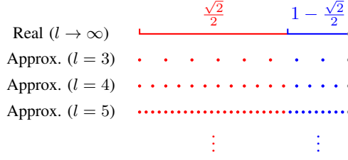
Figure S.1: Approximating the probability distribution (\frac{\sqrt{2}}{2}, 1 - \frac{\sqrt{2}}{2}) over \{m_1, m_2\} by random l bits (i.e., l -bit ciphertexts/seeds).
