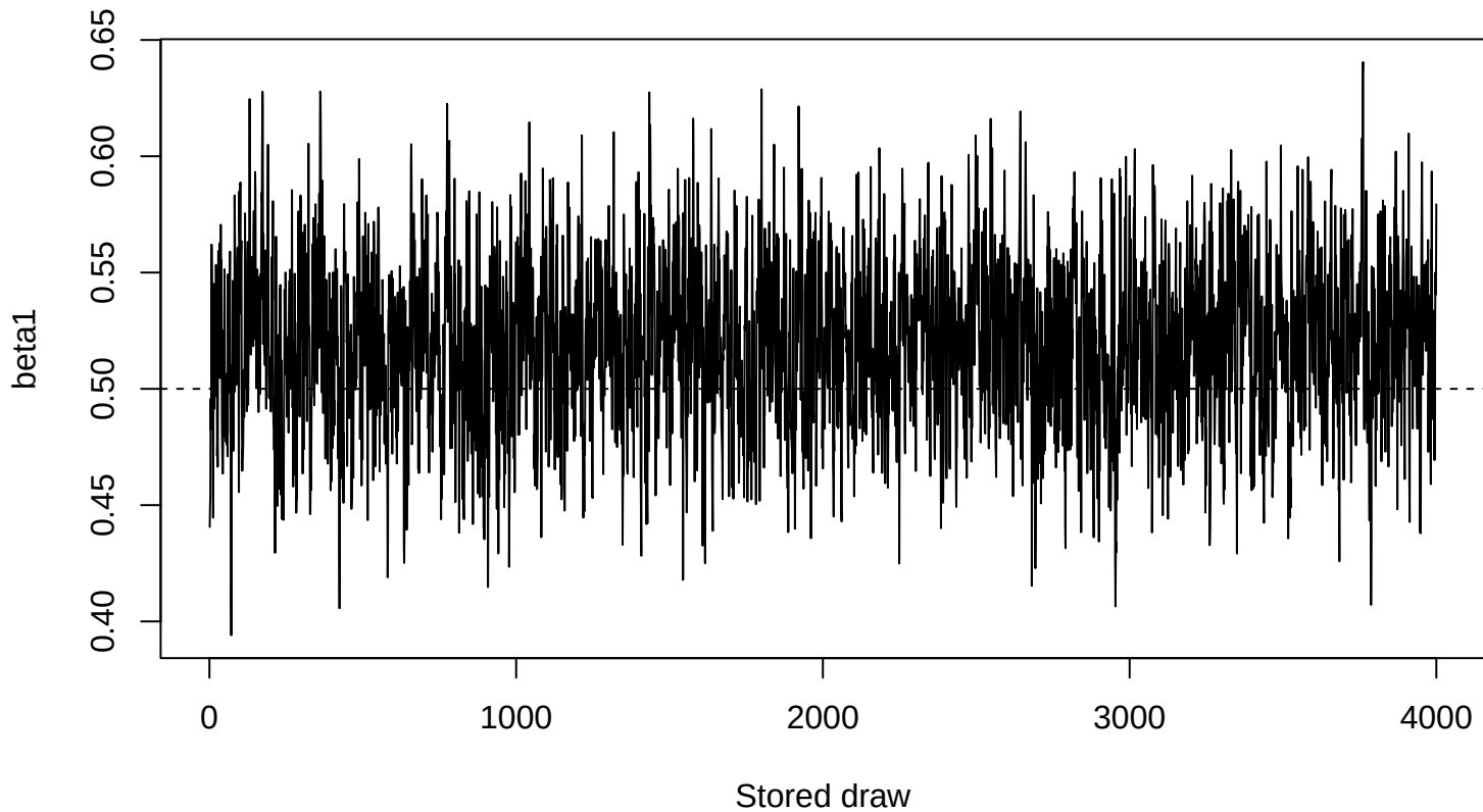
S4A rep 01: beta1 trace
