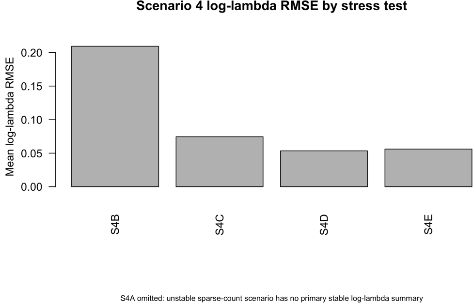
Figure 4: Average log-lambda RMSE across S4B–S4E. S4A is omitted because it is the sparse-count instability scenario and has no primary stable log-lambda summary in the overall table.
