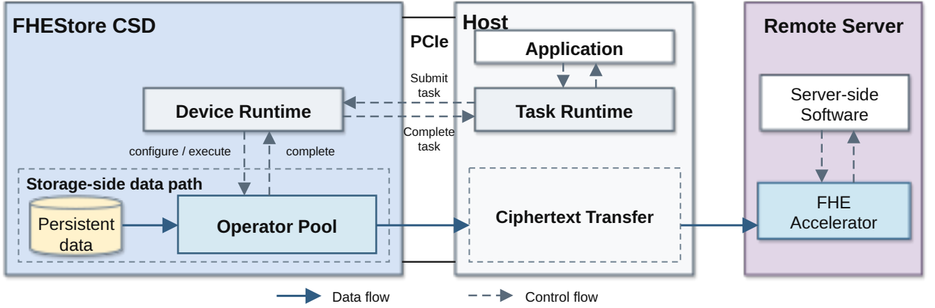
Figure 2: FHEStore architecture for FHE input preparation. Solid blue arrows denote data flow; dashed gray arrows denote control flow.
