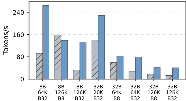
(a) HBM overflow throughput
