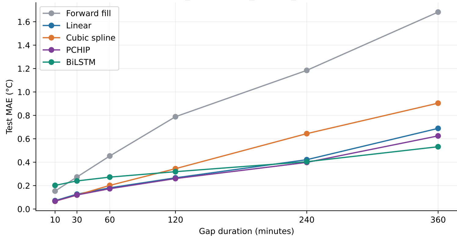
A_multivariate_context_12h
