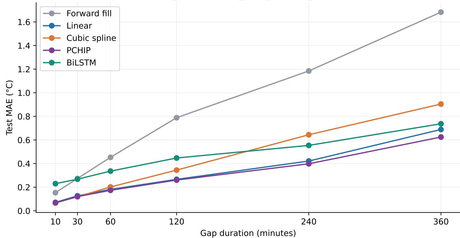
A_temperature_only_context_12h
