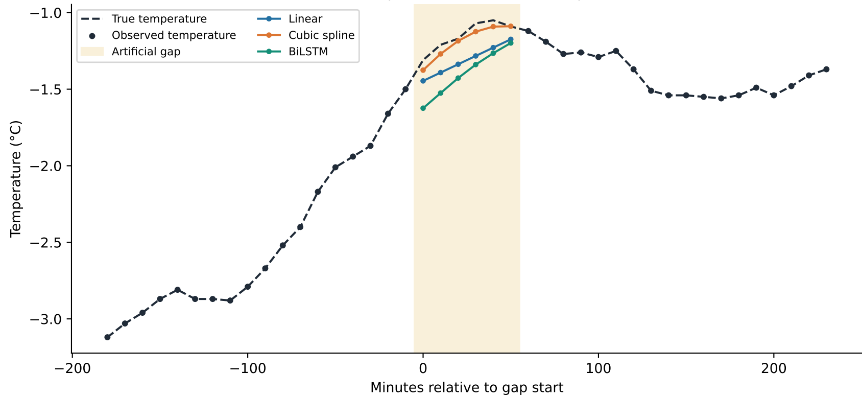
60-minute gap | 2016-01-04 13:40:00 | scenario B
