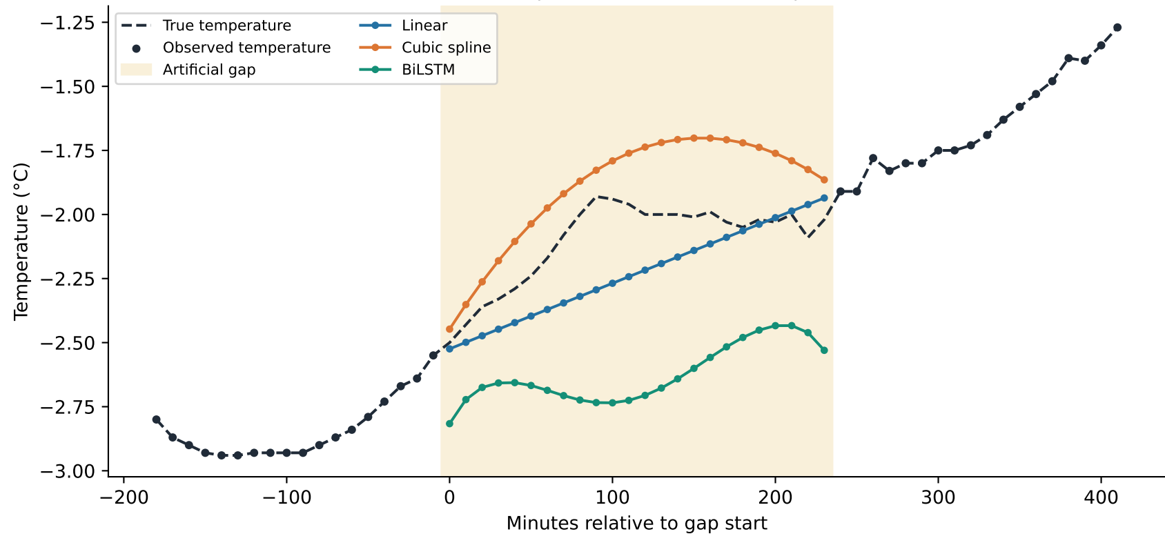
240-minute gap | 2016-01-03 03:50:00 | scenario B
