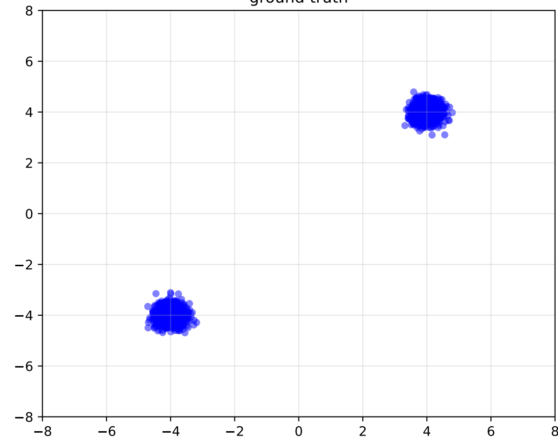
ground truth
