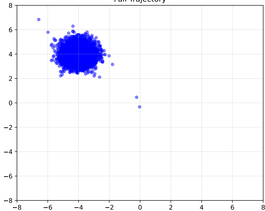
Full Trajectory
