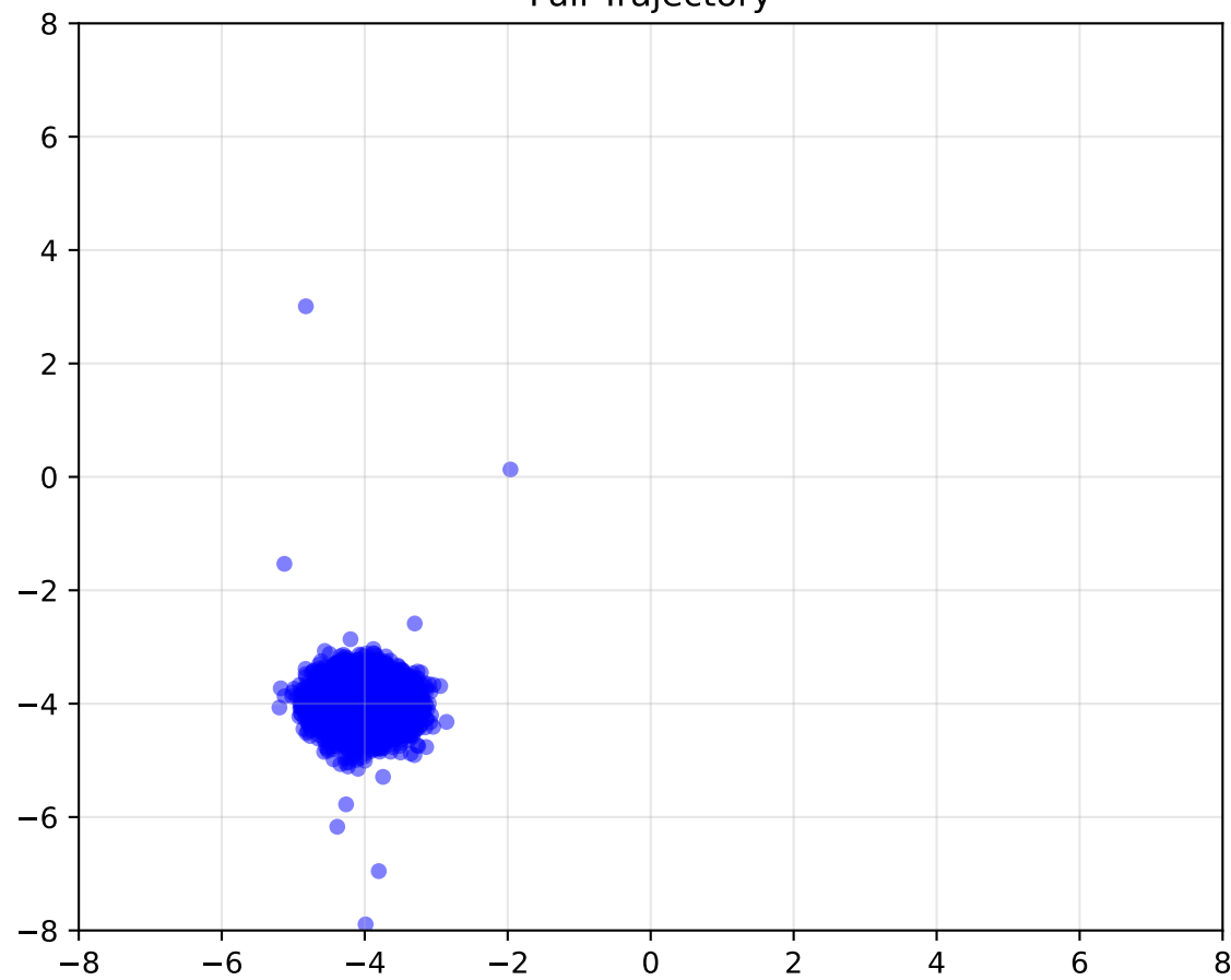
Full Trajectory
