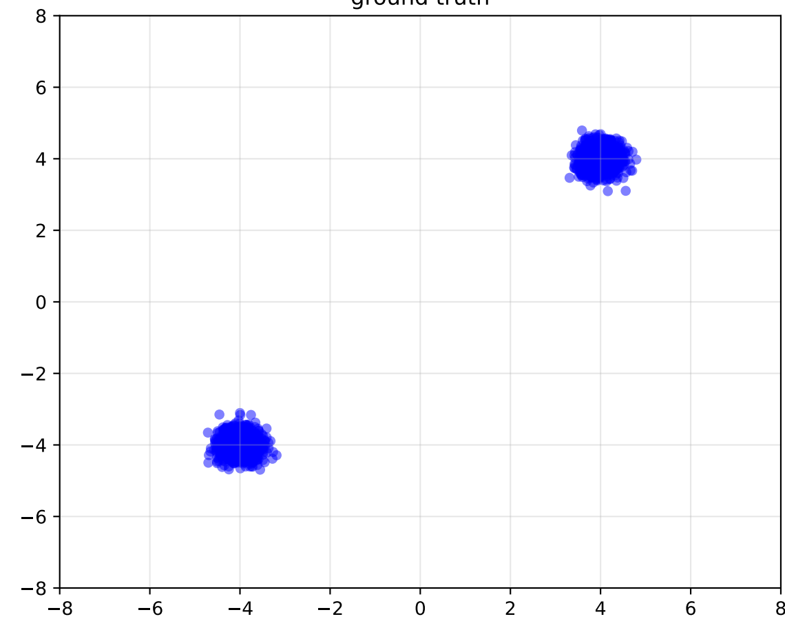
ground truth
