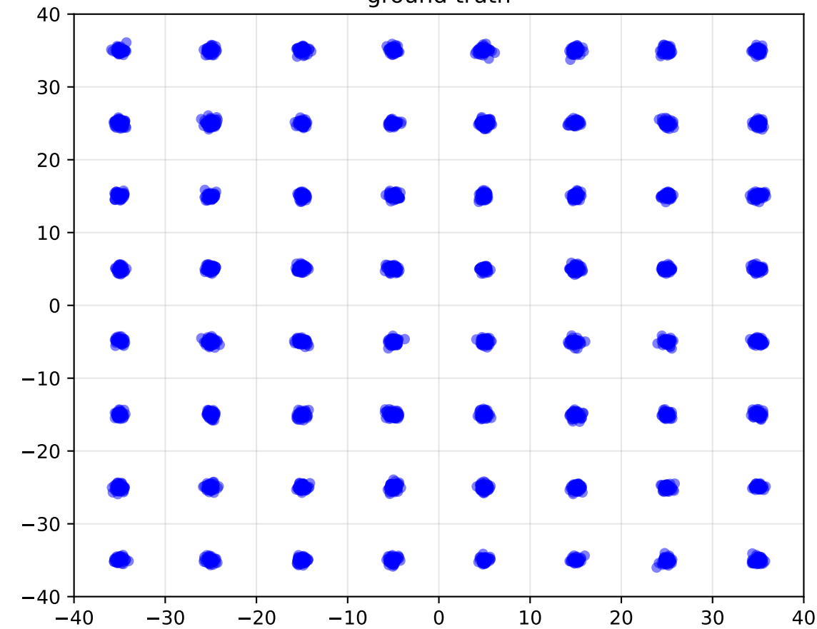
ground truth
