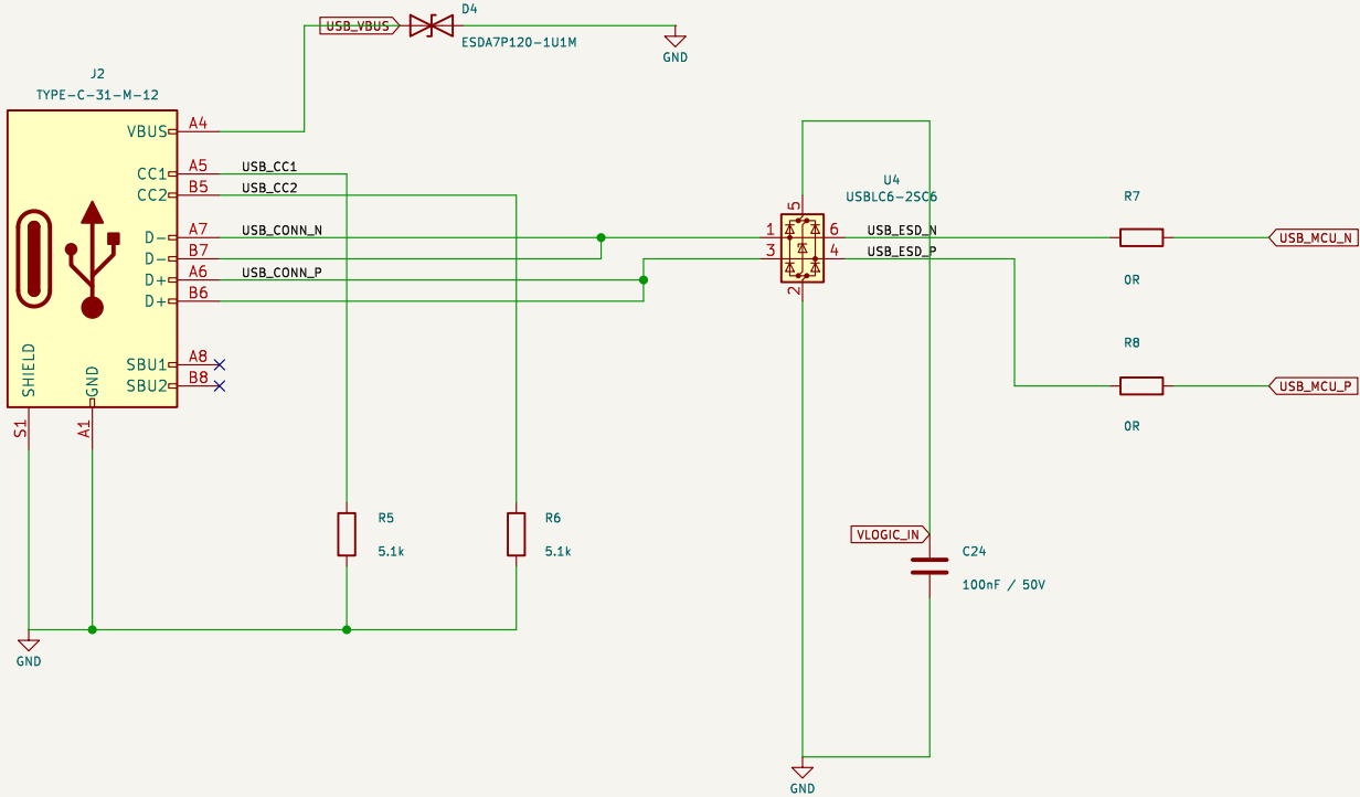
USB-C termination and ESD
