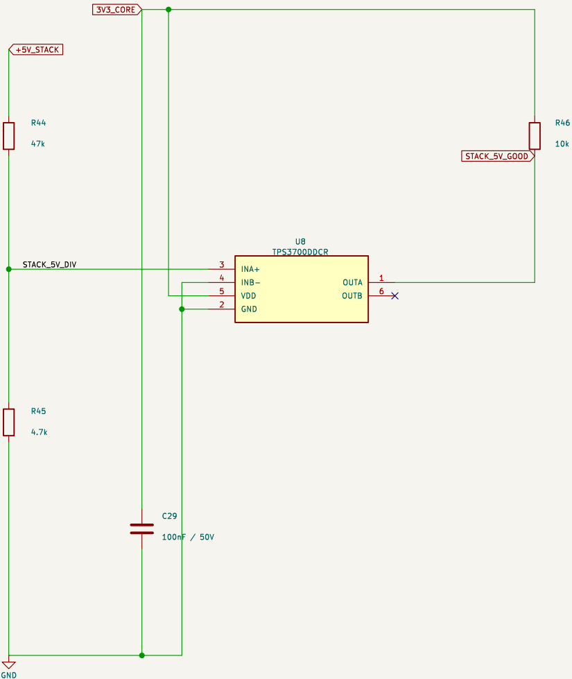
Stack 5 V health monitor
