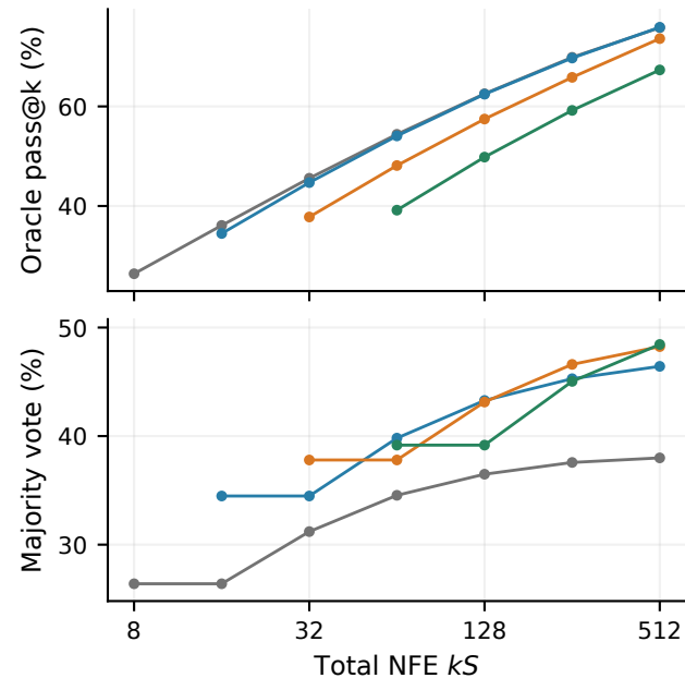
GSM8K ELF-B · pre-NFT
