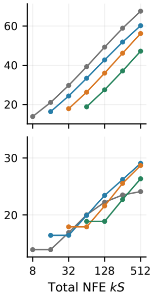
MATH500 Pre-NFT
