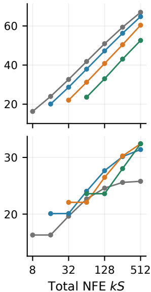
MATH500 Post-NFT
