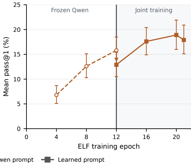
MATH500
