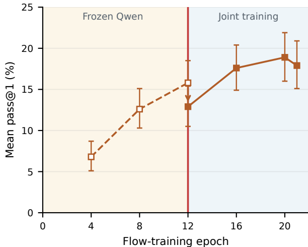
MATH500
