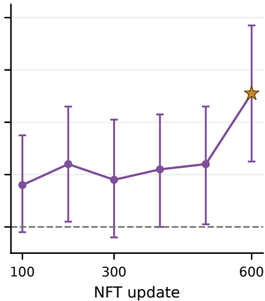
MATH500 / ELF-L
