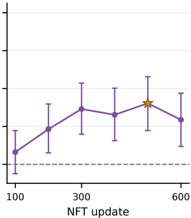
GSM8K / ELF-L
