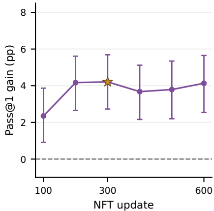
GSM8K / ELF-B
