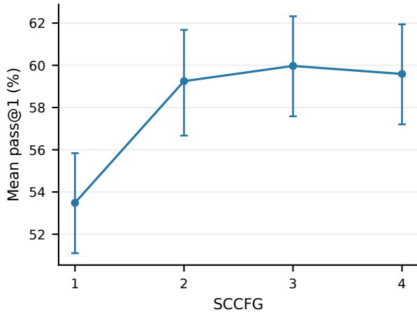
GSM8K / ELF-L
