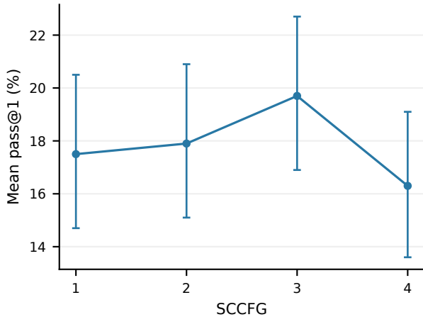
MATH500 / ELF-L
