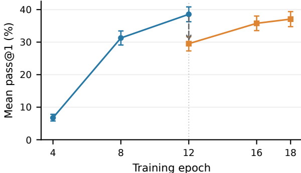
GSM8K / ELF-L · pre-NFT
