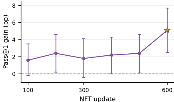
MATH500 / ELF-L · NFT gain
